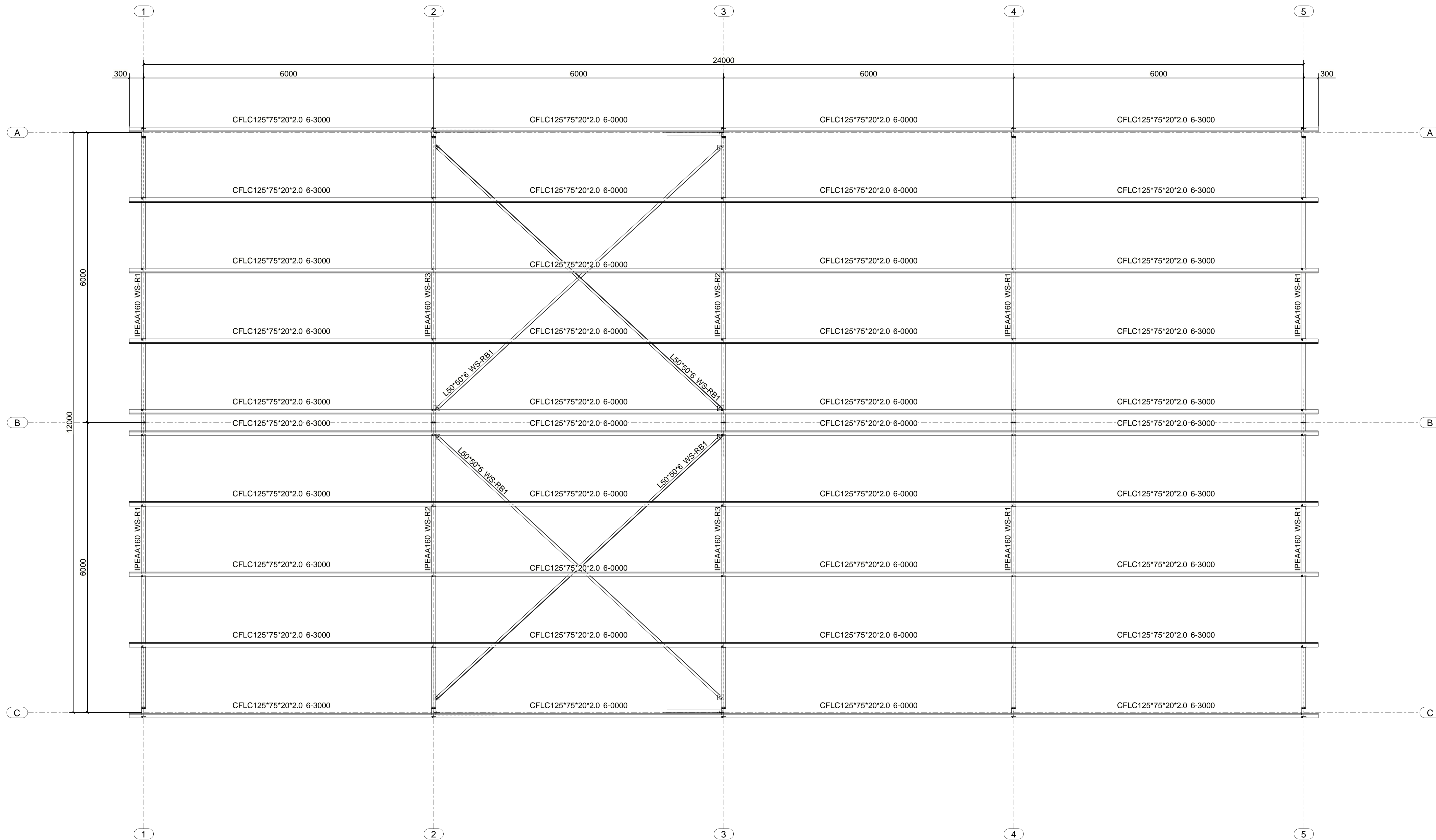
ROOF LAYOUT
