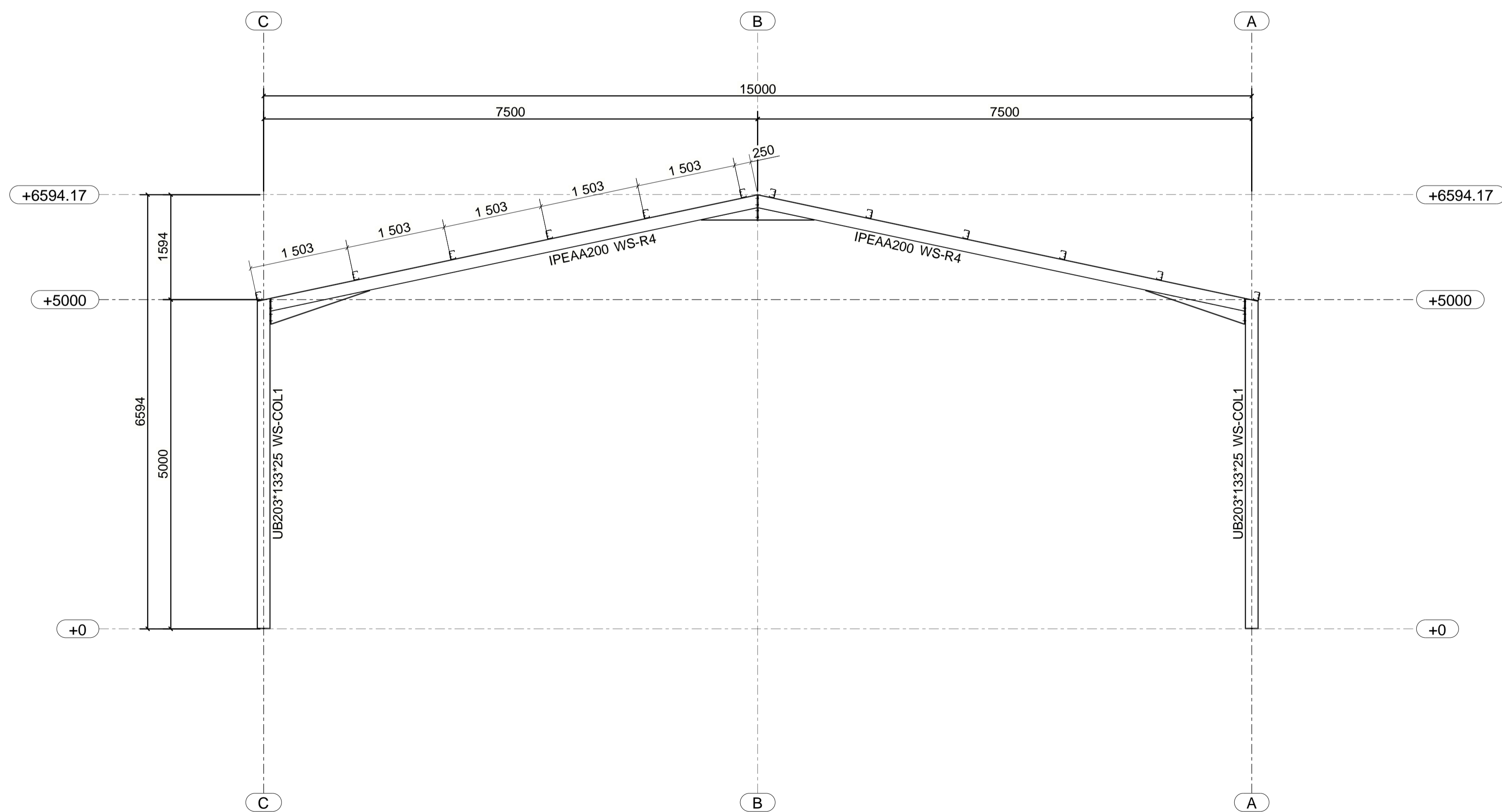
SECTION GRID 5
