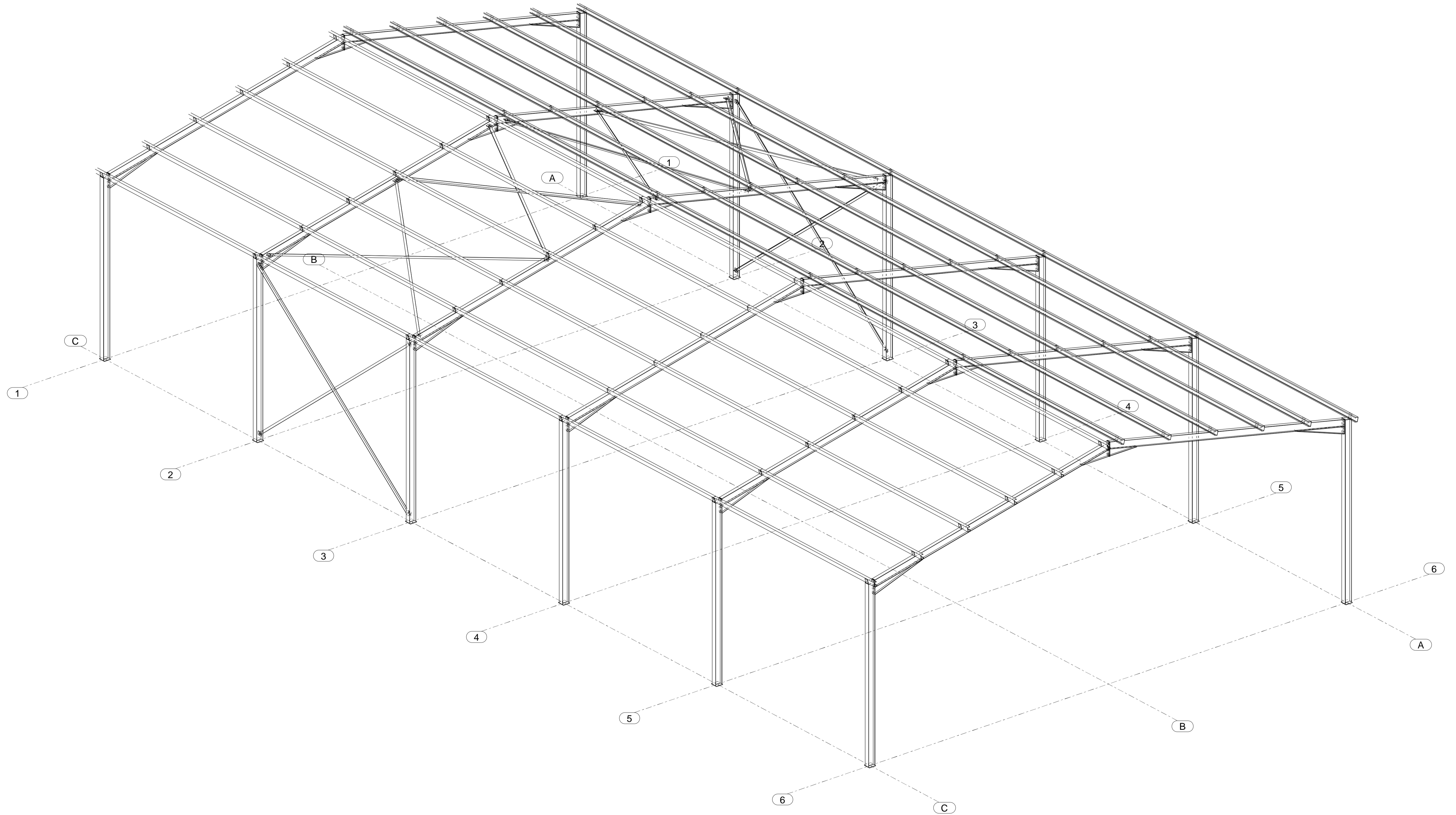
3D VIEW
