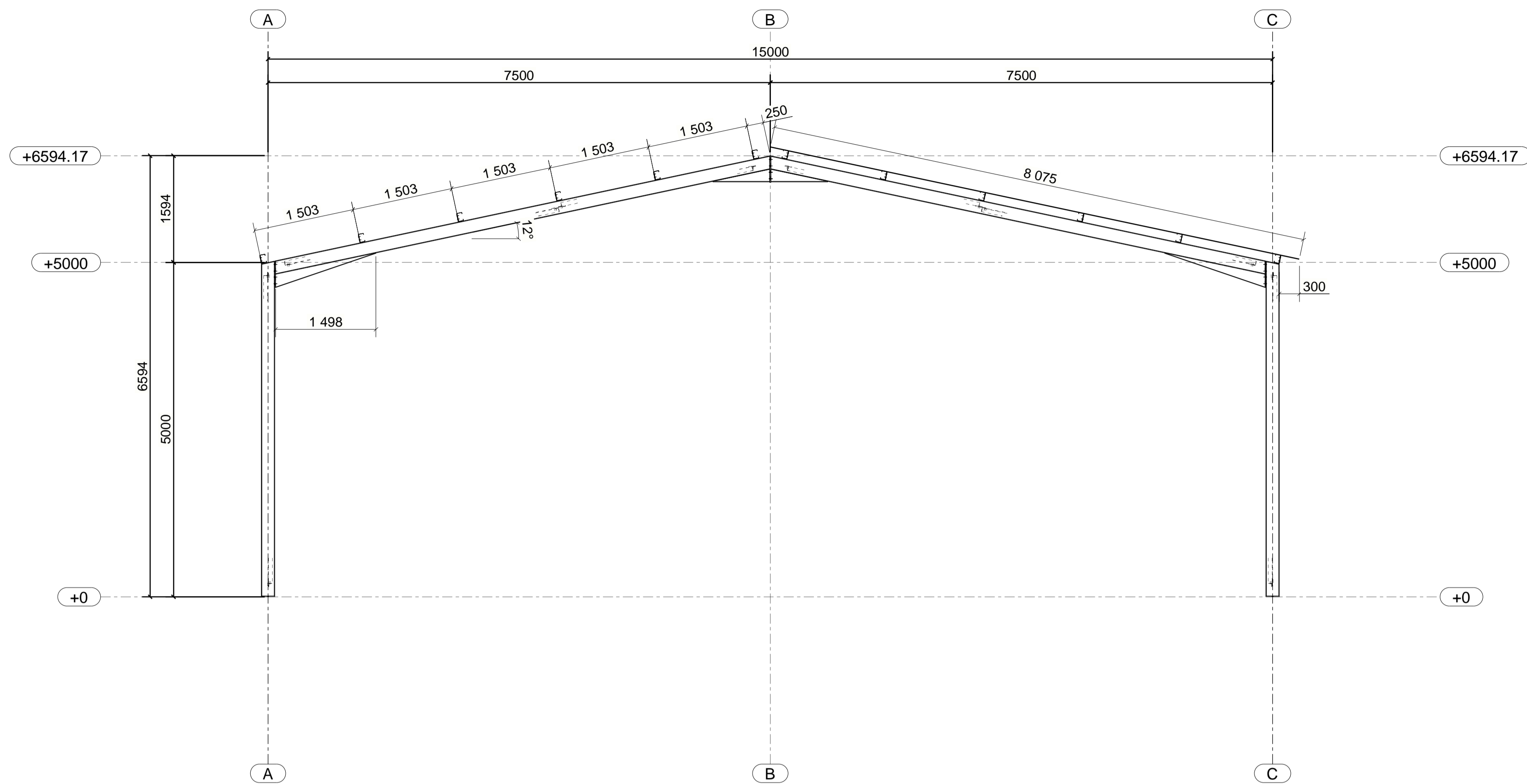
ELEV GRID 1
